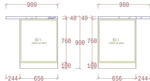
ELEVATION C
