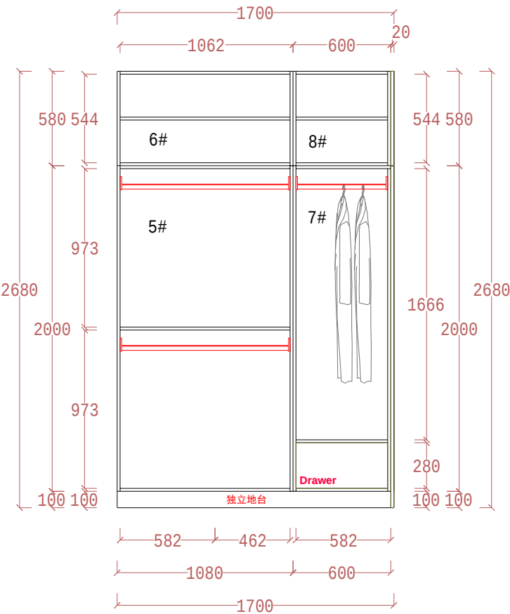
INNER VIEW B
