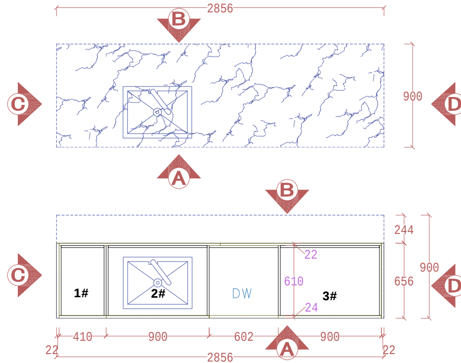
PLAN VIEW floor
