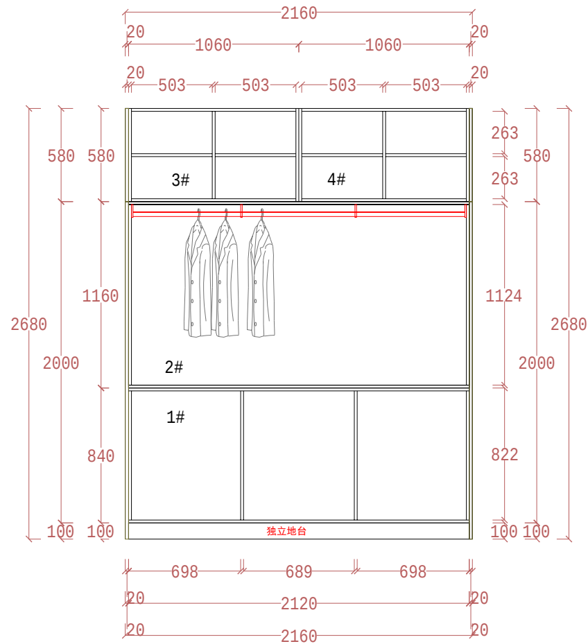
INNER VIEW A
