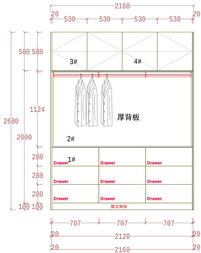
OUTSIDE VIEW A
