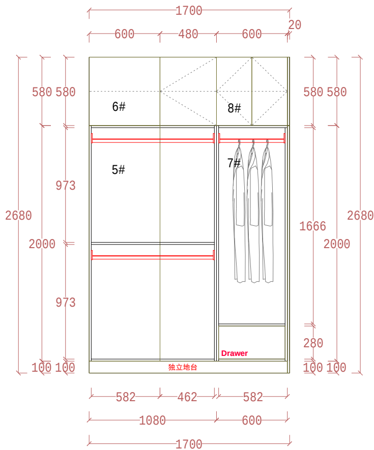
OUTSIDE VIEW B
