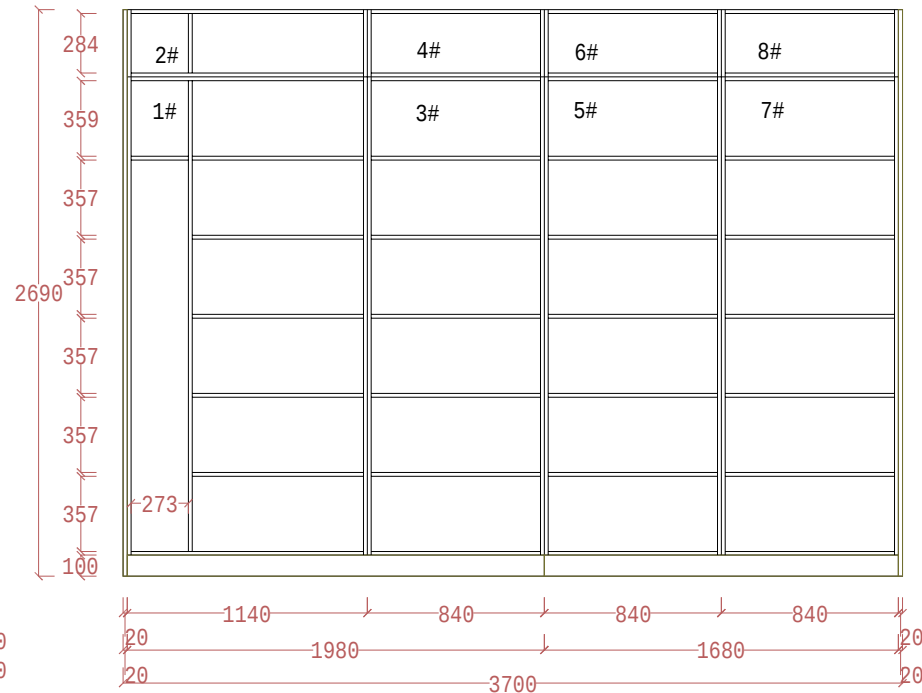
INNER VIEW
